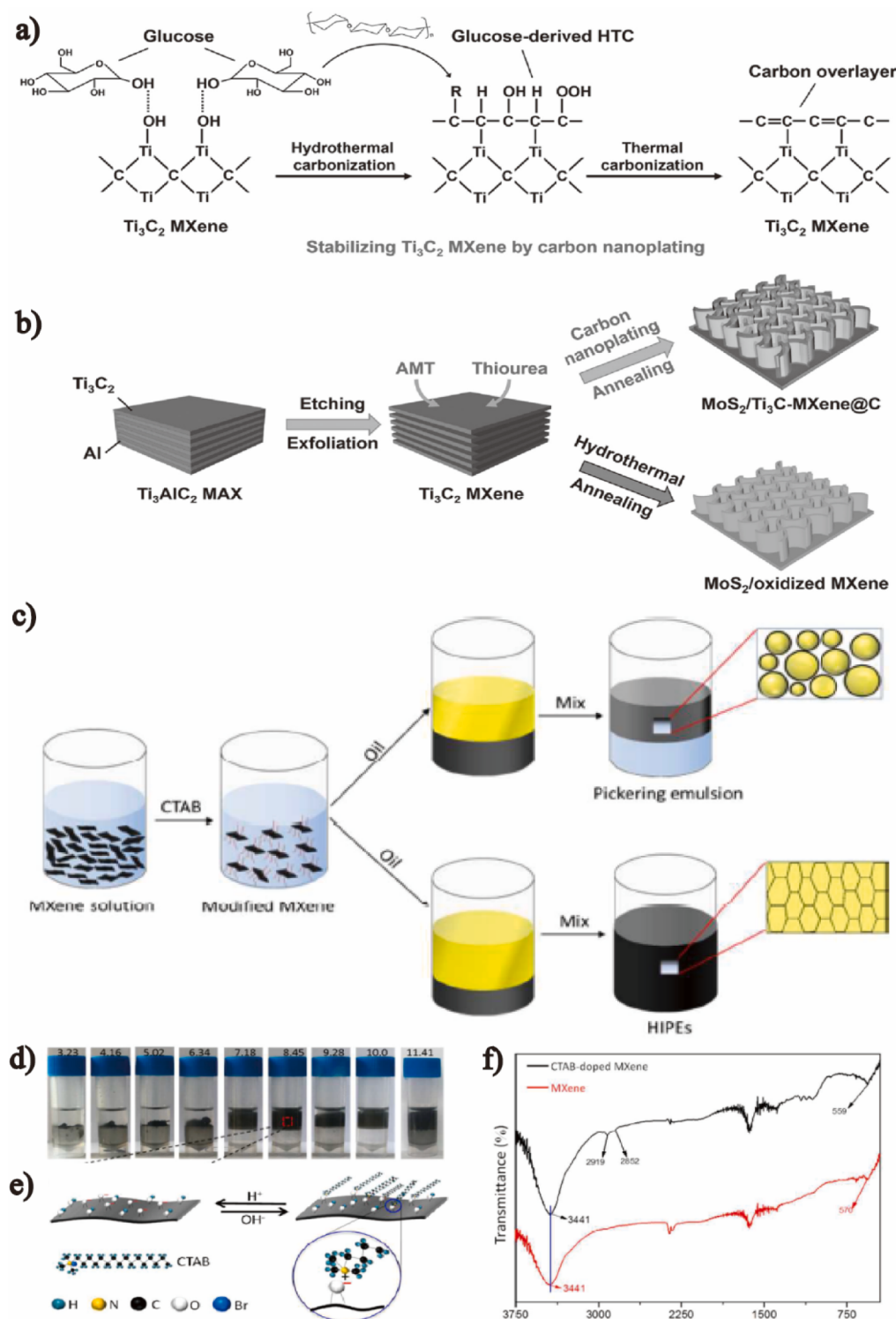
Fig. 9. (a) Schematic illustration of preparing carbon nanoplating on the surface of \text{Ti}_3\text{C}_2 . This process involves the adsorption of glucose molecules, the formation of hydrothermal carbon, and thermal carbonization at high temperatures. Reprinted with permission.[47] Copyright 2017, Wiley-VCH. (b) The preparation process of \text{MoS}_2/\text{Ti}_3\text{C}_2\text{-MXene@C} and \text{MoS}_2/\text{oxidized MXene} hybrid systems. \text{Ti}_3\text{C}_2\text{T}_x is rapidly transformed into \text{TiO}_2 during the reaction in the absence of carbon nanoplating. Reprinted with permission.[47] Copyright 2017, Wiley-VCH. (c) Schematic illustration of preparing oil-in-water Pickering emulsions and high internal phase Pickering emulsions (HIPEs) with CTAB-modified \text{Ti}_3\text{C}_2 (water molecules: blue, dodecane molecules: yellow). Reprinted with permission.[46] Copyright 2018, The Royal Society of Chemistry. (d) The effect of pH in an aqueous phase on emulsion stability with a fixed addition of CTAB and \text{Ti}_3\text{C}_2 . Reprinted with permission.[46] Copyright 2018, The Royal Society of Chemistry. (e) The interaction between CTAB and \text{Ti}_3\text{C}_2 at different pH. Reprinted with permission.[46] Copyright 2018, The Royal Society of Chemistry. (f) The FTIR spectra of CTAB-modified \text{Ti}_3\text{C}_2 . Reprinted with permission.[46] Copyright 2018, The Royal Society of Chemistry.
