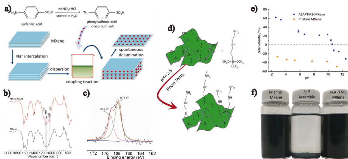
Fig. 6. (a) Schematic illustration for surface modification of multilayer \text{Ti}_3\text{C}_2\text{T}_x with aryl diazonium salts. Reprinted with permission. [66] Copyright 2016, Elsevier. (b) The FTIR spectra of \text{Ti}_3\text{C}_2 before and after modified by aryl diazonium salts. Reprinted with permission. [66] Copyright 2016, Elsevier. (c) The S 2p XPS spectrum of \text{Ti}_3\text{C}_2 after modification. Reprinted with permission. [66] Copyright 2016, Elsevier. (d) Schematic illustration for surface modification of \text{Ti}_3\text{C}_2\text{T}_x with [3-(2-aminoethylamino)propyl]trimethoxysilane (AEAPTMS) coupling agent. Reprinted with permission. [70] Copyright 2020, Wiley-VCH. (e) Surface charge of \text{Ti}_3\text{C}_2\text{T}_x before and after AEAPTMS modification at different pH values. Reprinted with permission. [70] Copyright 2020, Wiley-VCH. (f) Self-assembly of \text{Ti}_3\text{C}_2\text{T}_x formed by mixing MXene with opposite surface charge. Reprinted with permission. [70] Copyright 2020, Wiley-VCH.
