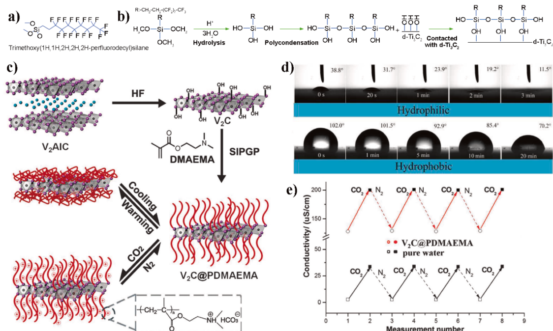
Fig. 7. (a) The molecular structure of PFDTMS. Reprinted with permission.[67] Copyright 2018, The Royal Society of Chemistry. (b) Schematic illustration of grafting PFDTMS onto \text{Ti}_3\text{C}_2 surface. Reprinted with permission.[67] Copyright 2018, The Royal Society of Chemistry. (c) Schematic illustration of grafting PDMAEMA onto \text{V}_2\text{C} surface (C atom: gray white, V atom: purple, Al atom: blue). Reprinted with permission.[42] Copyright 2015, The Royal Society of Chemistry. (d) Time course contact angles of \text{Ti}_3\text{C}_2 film before and after modification. Reprinted with permission.[67] Copyright 2018, The Royal Society of Chemistry. (e) Conductivity changes of \text{V}_2\text{C}@PDMAEMA suspension measured at 25^\circ\text{C} during repeated \text{CO}_2 uptake-release process. The concentration of aqueous suspension is 3.0 \text{ mg mL}^{-1} . The average conductivity value was calculated from three measurements. Reprinted with permission.[42] Copyright 2015, The Royal Society of Chemistry.
