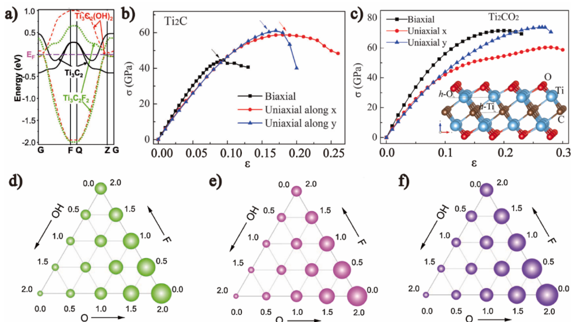
Fig. 2. (a) Calculated band structure of monolayer \text{Ti}_3\text{C}_2 with -\text{OH} and -\text{F} functional groups and without termination, corresponding to semiconductor and metal characteristics, respectively. Reprinted with permission.[5] Copyright 2011, Wiley-VCH. (b) Calculated stress-strain curves of \text{Ti}_2\text{C} without termination. These points marked by arrows are the strain at the beginning of instability. Reprinted with permission.[53] Copyright 2015, The Royal Society of Chemistry. (c) Calculated stress-strain curves of \text{Ti}_2\text{C} with -\text{O} functional group. The inset shows the atomic structure of \text{Ti}_2\text{CO}_2 with the functional group distribution in the most energetically favorable positions. Reprinted with permission.[53] Copyright 2015, The Royal Society of Chemistry. The relative stability of (d) \text{Ti}_3\text{C}_2 , (e) \text{Ti}_2\text{C} , (f) \text{Nb}_4\text{C}_3 with mixed functional groups ( -\text{F} , -\text{O} , and -\text{OH} ). The larger the bubble size, the stronger the relative stability of MXenes. Reprinted with permission.[58]. Copyright 2018, American Chemical Society.
