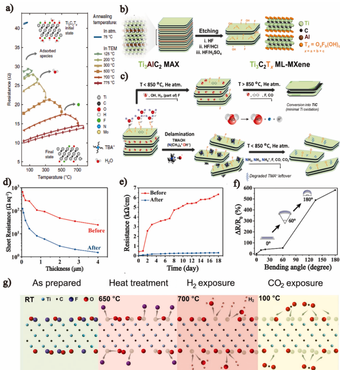
Fig. 4. (a) The effect of in-situ vacuum annealing temperature on Ti_3C_2T_x resistance. The curves with different colors correspond to different vacuum annealing processes, including heating and cooling stages. The atomic structures of Ti_3C_2T_x in the initial and final states are shown as insets. Reprinted with permission.[9] Copyright 2019, Springer Nature Publishing. (b) Multilayer Ti_3C_2T_x MXene synthesized with different etchants such as HF, HF/HCl, or HF/H 2 SO 4 . Reprinted with permission.[65] Copyright 2019, American Chemical Society. (c) The variation of Ti_3C_2T_x treated by different approaches during heat treatment. MXenes undergo partial oxidation and phase transition in a He environment when the temperature exceeds 850 ^{\circ}C . The oxidation is caused by hydroxyl radicals ( HO\cdot ) and superoxide anions ( O_2^- ) produced during heat treatment. Reprinted with permission.[65] Copyright 2019, American Chemical Society. (d) Effect of heat treatment on the conductivity of Ti_3C_2T_x films with different thicknesses. Reprinted with permission.[22] Copyright 2020, The Royal Society of Chemistry. (e) Stability of Ti_3C_2T_x films before and after heat treatment in an atmospheric environment. Reprinted with permission.[22] Copyright 2020, The Royal Society of Chemistry. (f) Response of heat-treated film to bending. Reprinted with permission.[22] Copyright 2020, The Royal Society of Chemistry. (g) Schematic illustration of surface termination changes distributed on Ti_3C_2T_x nanosheets under different treatment stages and environmental atmosphere. Reprinted with permission.[29] Copyright 2019, Wiley-VCH.
