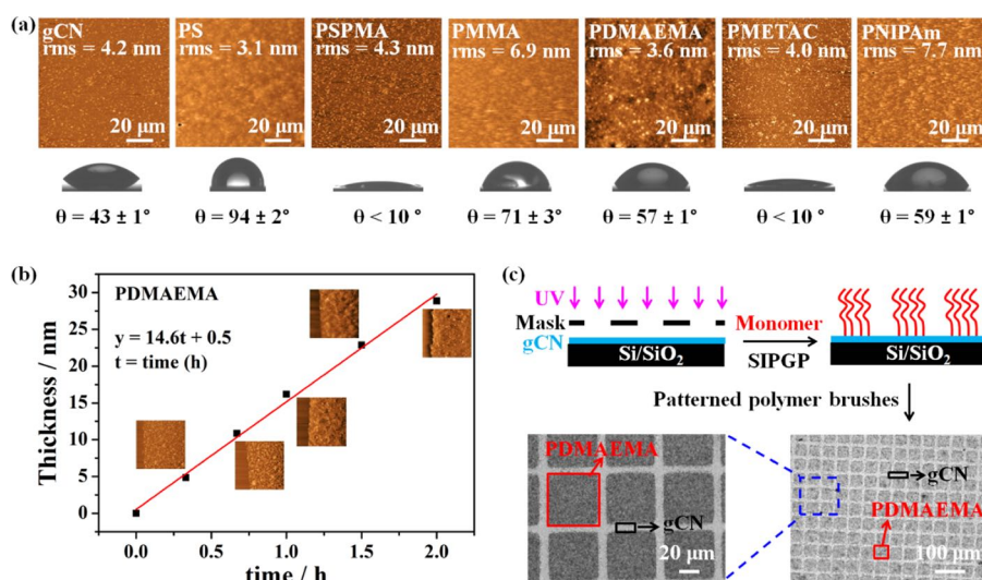
Figure 3. (a) AFM images and water contact angle of gCN and polymer-modified gCN. (b) Thickness evolution of polymer brushes grafted on gCN as a function of polymerization time for PDMAEMA brushes (PDMAEMA as a model system). (c) Schematic illustration and optical photographs of patterned PDMAEMA brushes on a spin-coated gCN film.
