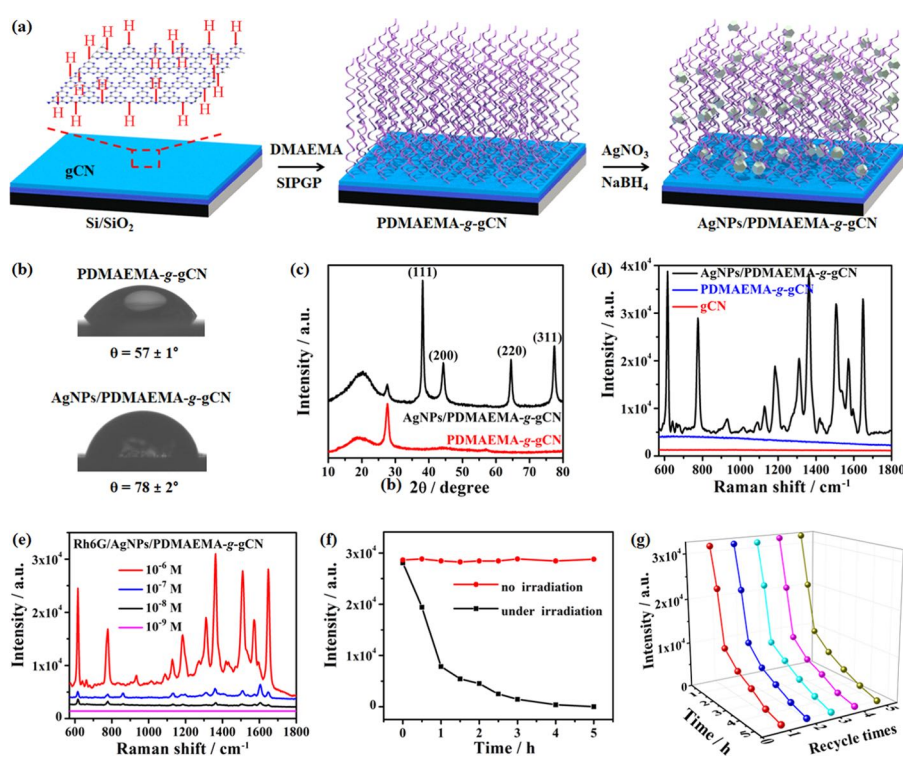
Figure 5. (a) Schematic illustration of the fabrication of PDMAEMA-g-gCN by SIPGP and subsequent immobilization of AgNPs on PDMAEMA-g-gCN. (b) Contact angles and (c) XRD spectra of PDMAEMA-g-gCN and AgNPs/PDMAEMA-g-gCN. (d) SERS spectra of 10^{-6} M Rh6G on native, PDMAEMA-g-gCN, and AgNPs/PDMAEMA-g-gCN. (e) SERS spectra for AgNPs/PDMAEMA-g-gCN probed with different concentrations of Rh6G from 10^{-6} to 10^{-9} M in ethanol. (f) SERS intensity plot for the band at 1649\text{ cm}^{-1} vs time without and with visible light irradiation to completely remove the Rh6G from the AgNPs/PDMAEMA-g-gCN layer. (g) The SERS intensities at 1649\text{ cm}^{-1} for visible light-assisted degradation of 10^{-6} M Rh6G on AgNPs/PDMAEMA-g-gCN for repeatable usage up to five times.
