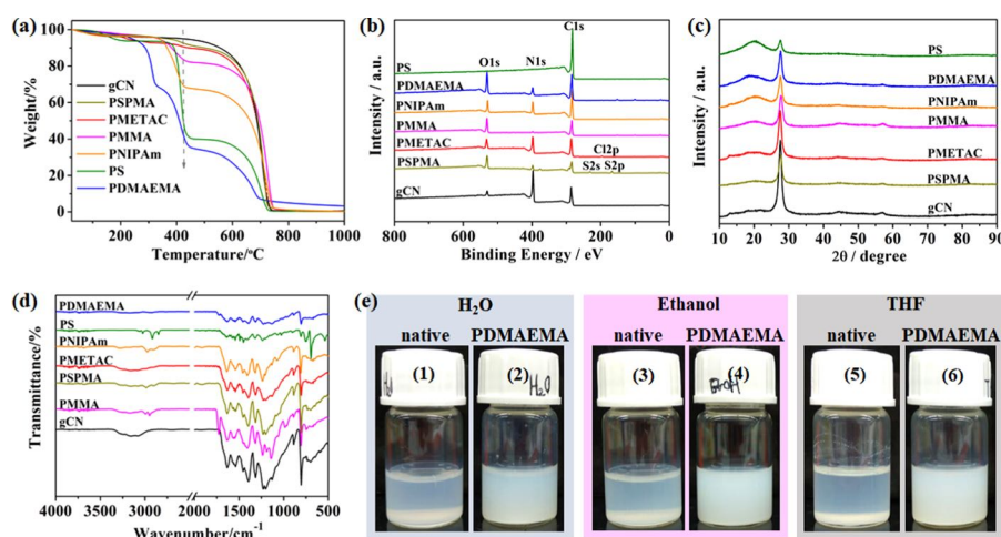
Figure 2. (a) TGA curves, (b) XPS spectra, (c) XRD patterns, and (d) FTIR spectra of native gCN and polymer brush-modified gCN. (e) The dispersibility of gCN (1, 3, 5) and PDMAEMA-g-gCN (2, 4, 6) in H 2 O, ethanol, and THF after 3 months, respectively. The concentrations of gCN and PDMAEMA-g-gCN in solvent are both 3 mg mL -1 .
