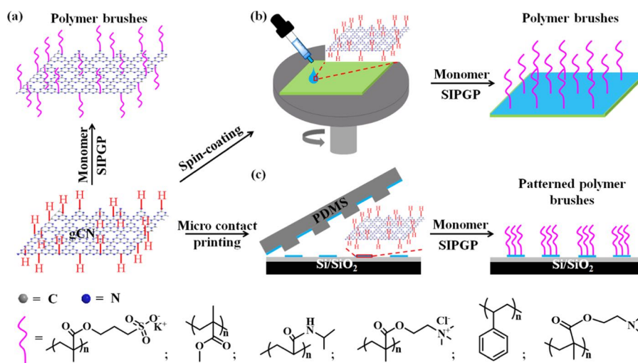
Figure 1. Schematic illustration of the preparation of polymer brushes on gCN particles (a), spin-coated gCN film (b), and microcontact printing gCN patterns (c).
